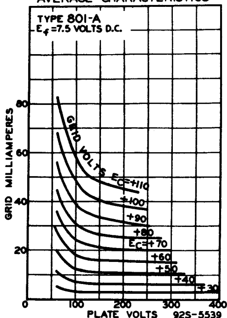
AVERAGE CHARACTERISTICS
